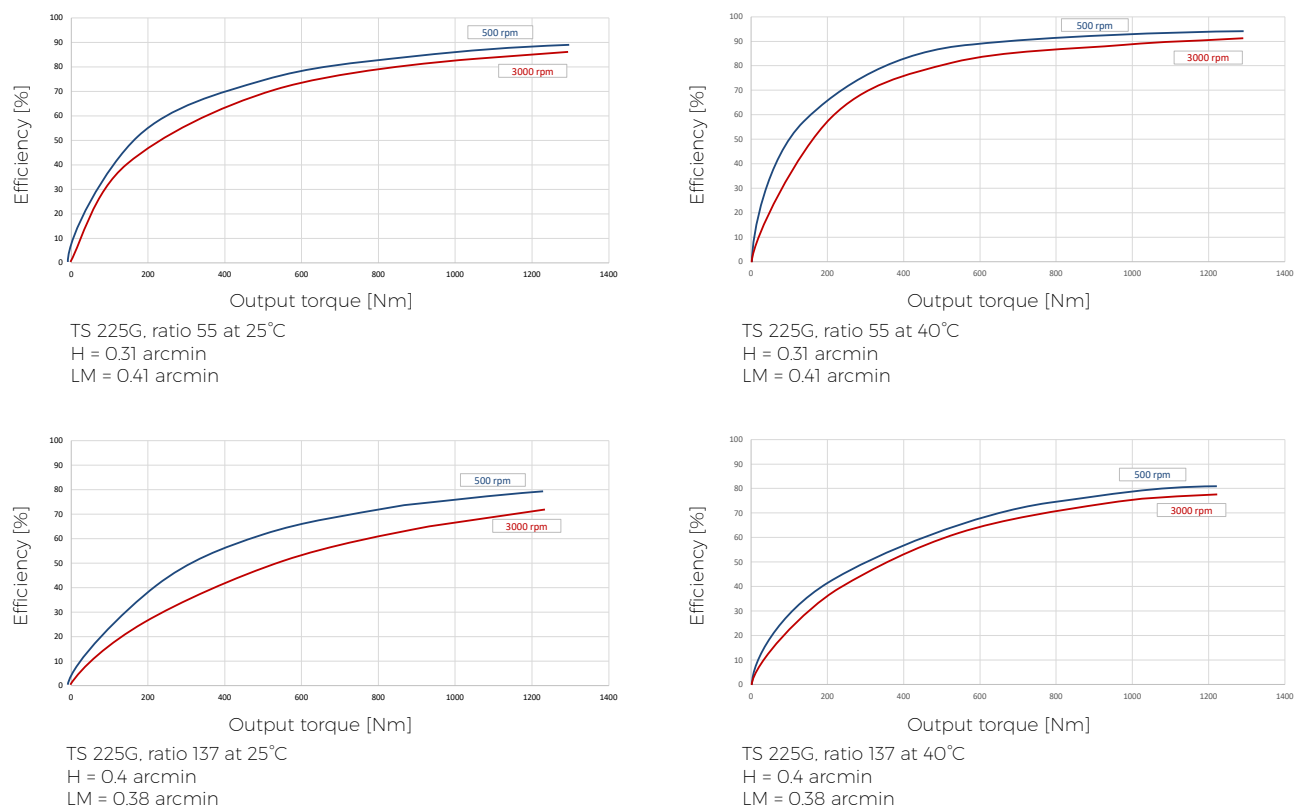
Fig. 3.13: Efficiency charts
