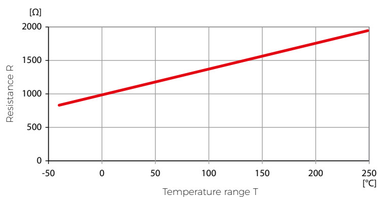
Fig. 8.5k: Resistance / Temperature PT 1000
