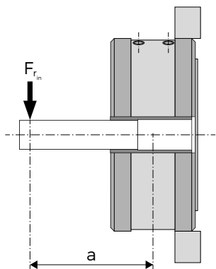
Fig. 3.12a: Radial load of the T, E, H series input shaft
