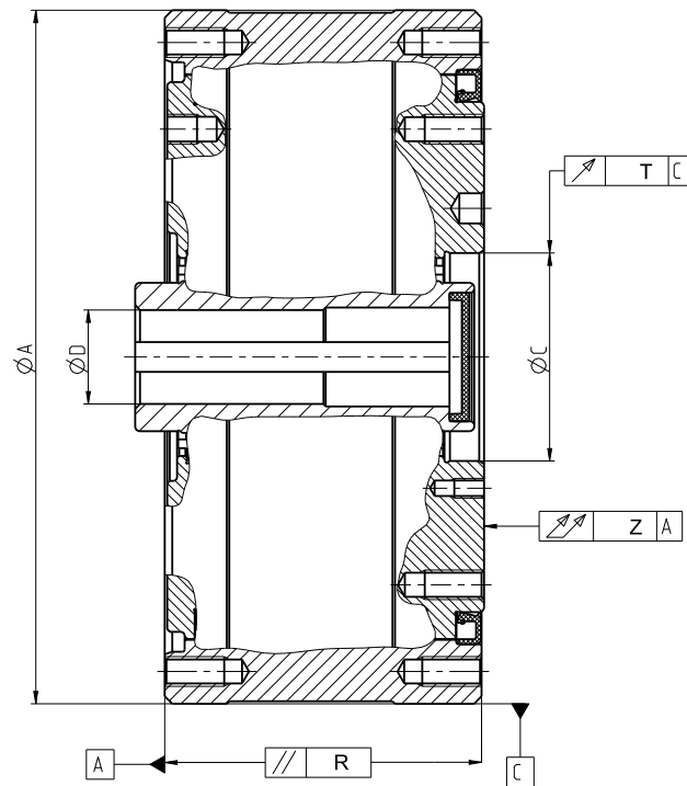
Fig. 5.1.5a: Tolerances of circumferential and face runout for direct connection of TwinSpin® high precision reduction gears with servomotor in accordance with DIN 42955 R
