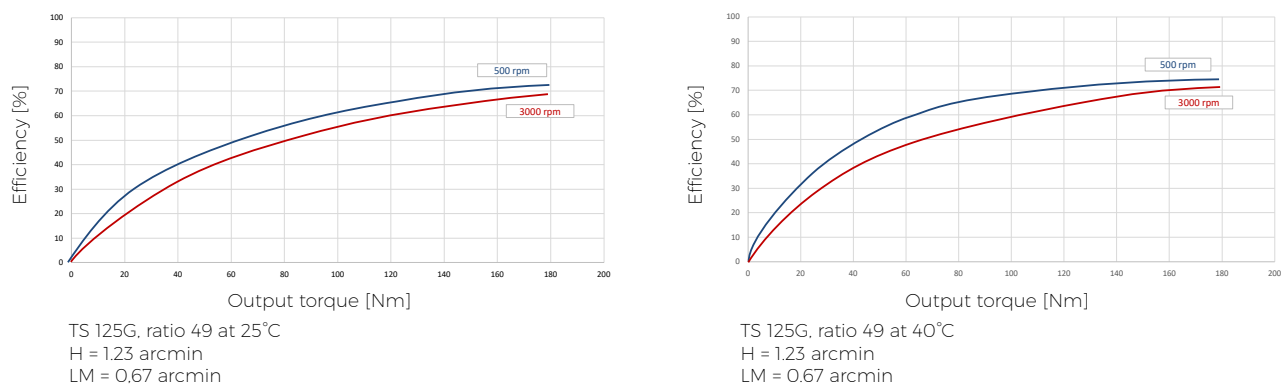
Fig. 3.14: Efficiency charts
