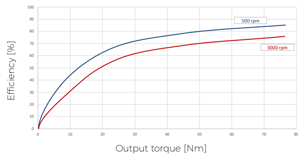
TS 85G, ratio 63 at 40°C H = 1.01 arcmin LM = 0.78 arcmin
