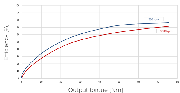
TS 85G, ratio 79 at 25°C H = 0.72 arcmin LM = 0.48 arcmin
