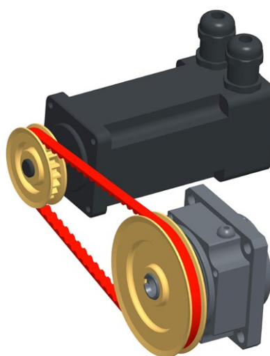
Fig. 5.4.1d: Example of the hollow-shaft version of the reduction gear use driven through a toothed belt
