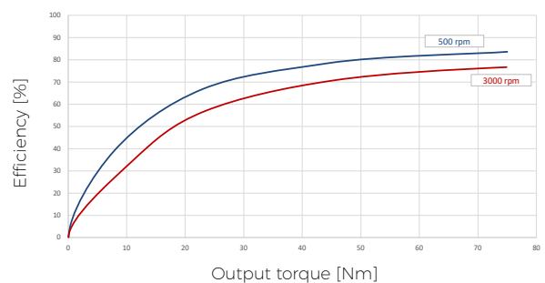
TS 85G, ratio 79 at 40°C H = 0.72 arcmin LM = 0.48 arcmin
