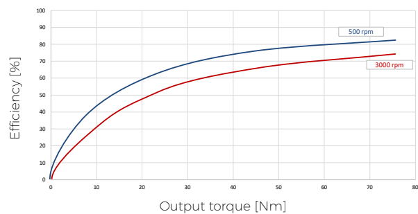
TS 85G, ratio 63 at 25°C H = 1.01 arcmin LM = 0.78 arcmin
